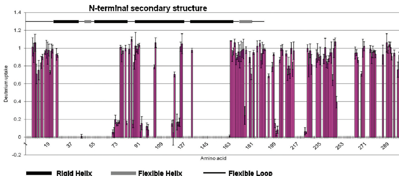
Figure 6. Extent of deuterium uptake of each amide of ApoE4 monomeric mutant after correcting for back-exchange (pink). Most of the amides in the C-terminus have high extent of deuterium uptake, indicating a flexible structure in this region. The extent of deuterium uptake in N-terminal region are consistent with the known secondary structure (top) (flexible loop, black line; flexible helix, gray box; rigid helix, black box). Note: the gaps correspond to missing information.
