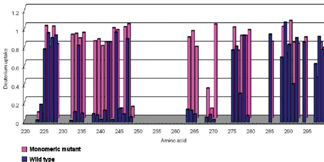
Figure 5. Extent of deuterium uptake of various amino acid residues in the C-terminal domain of ApoE4 (residue 220–299). Several residues of wild type (blue) have lower level ( <0.3D ) of deuterium uptake compared to the monomeric mutant (pink). Note: the gaps correspond to missing information.
