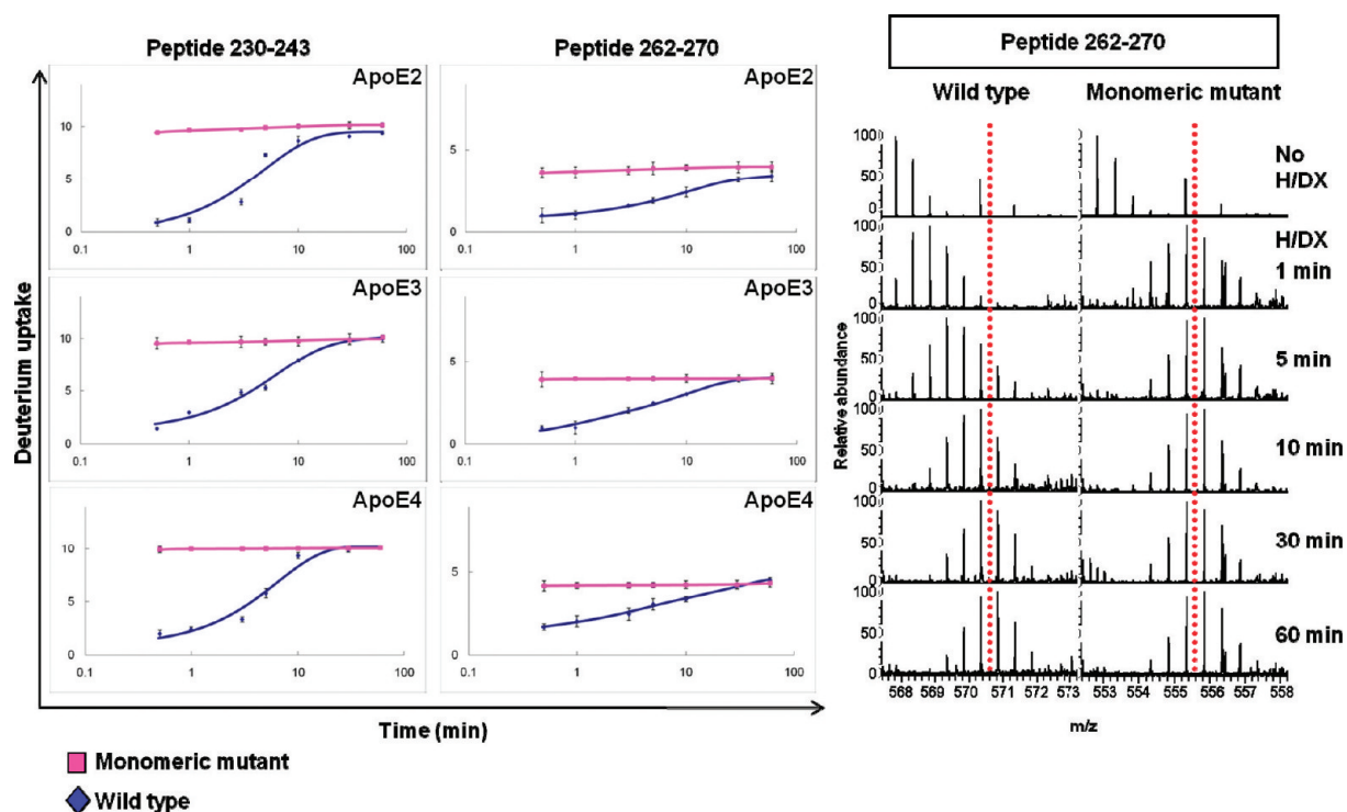
Figure 2. Comparison of H/DX kinetics of peptides 230–243 and 262–270 among all three isoforms (ApoE2, ApoE3, and ApoE4). An example of the mass spectra of peptide 262–270 of ApoE4 as a function of H/DX time is shown on the right (the red dotted line is a reference to guide the eye).
